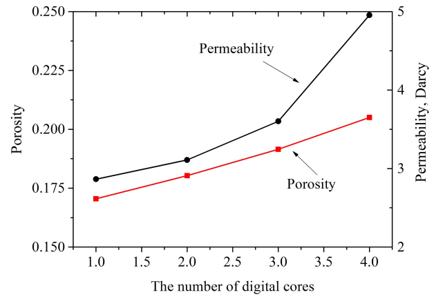
Fig. 5. Relationship between the permeabilities and the porosities.
