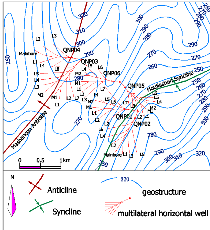
Fig. 2. Geostucture map of multilateral horizontal well control region.
