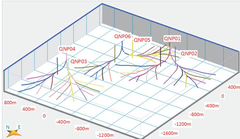
Fig. 1. Main bore and lateral branch patterns.
