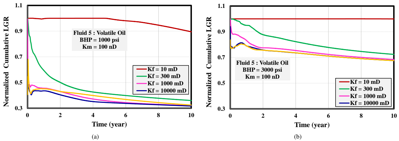
Fig. 6. Normalized cumulative liquid to gas ratio from reservoir of 100 nD permeability for various fracture permeability for fluid 5 at the volatile oil condition and operating at bottom hole pressure of (a) 1000 psia (b) 3000 psia.
