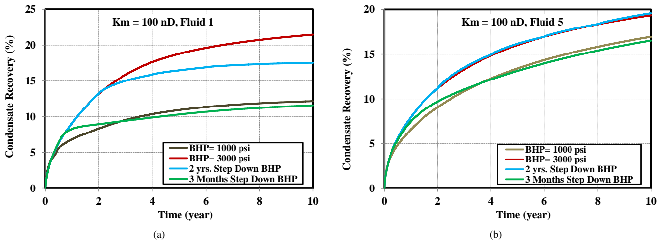
Fig. 14. Comparisons of condensate recoveries for constant and periodic step down of operating bottom hole pressure for (a) fluid 1 (b) fluid 5.
