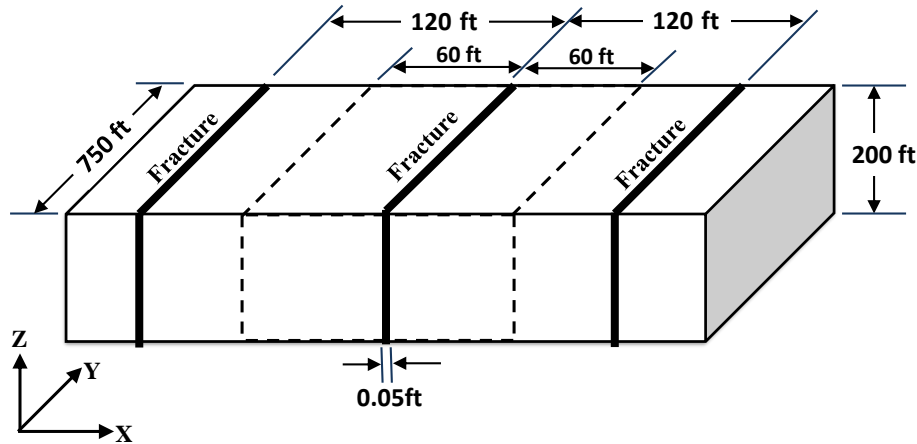
Fig. 4. Schematic diagram of reservoir model with multiple hydraulic fractures. Dotted portion is the simulated part of the model.
