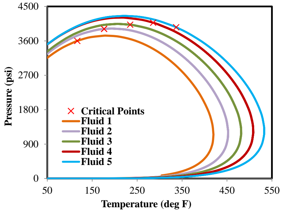
Fig. 3. Pressure-Temperature (PT) diagram showing the phase behavior of fluid 1 to fluid 5.
