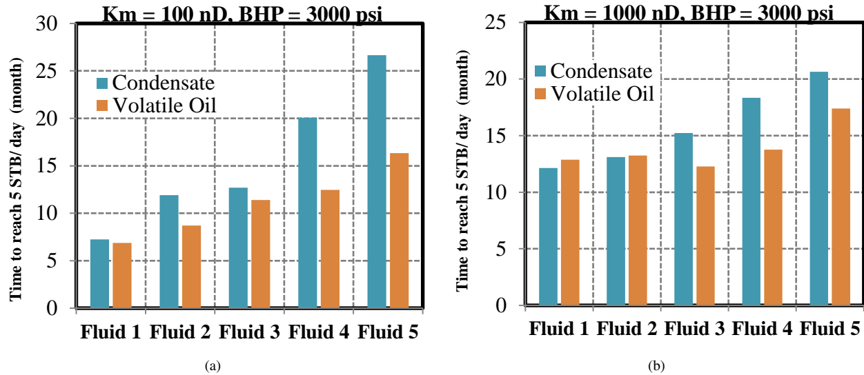
Fig. 11. Time to reach liquid flow rate of 5 STB/day/fracture for condensate and volatile oil reservoir with permeability of (a) 100 nD (b) 1000 nD.
