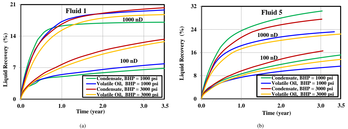
Fig. 8. Liquid recovery from 100 nD and 1000 nD permeability reservoirs with BHP of 1000 psia and 3000 psia for (a) fluid 1 (b) fluid 5.
