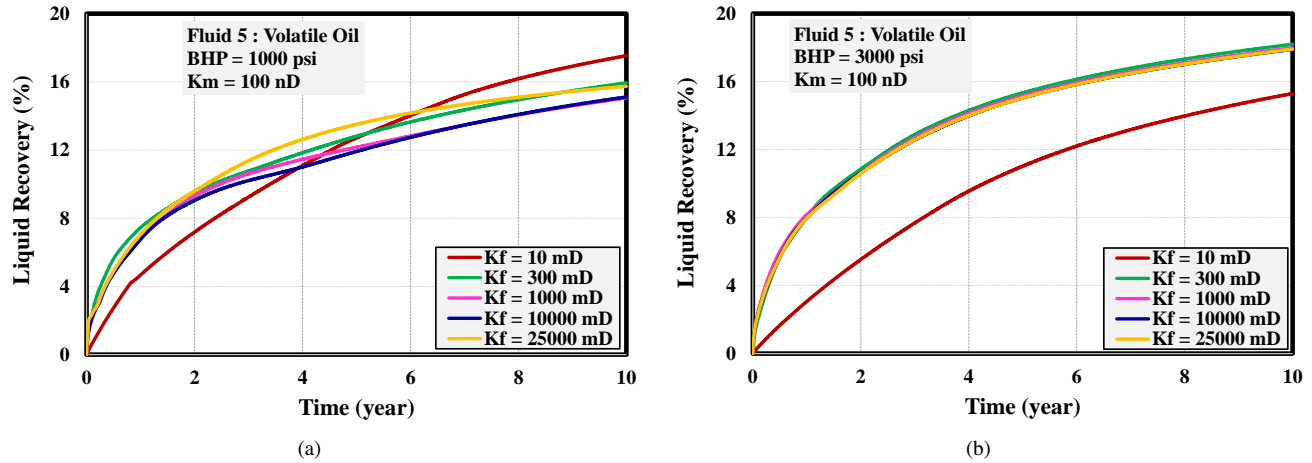
Fig. 5. Liquid recoveries from reservoir of 100 nD permeability for various fracture permeability for fluid 5 at the volatile oil condition and operating at bottom hole pressure of (a) 1000 psia (b) 3000 psia.
