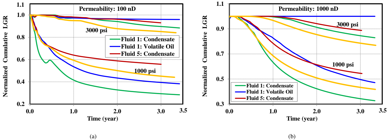
Fig. 12. Comparisons of normalized produced LGR for fluid 1 and fluid 5 in reservoir with permeability (a) 100 nD (b) 1000 nD.
