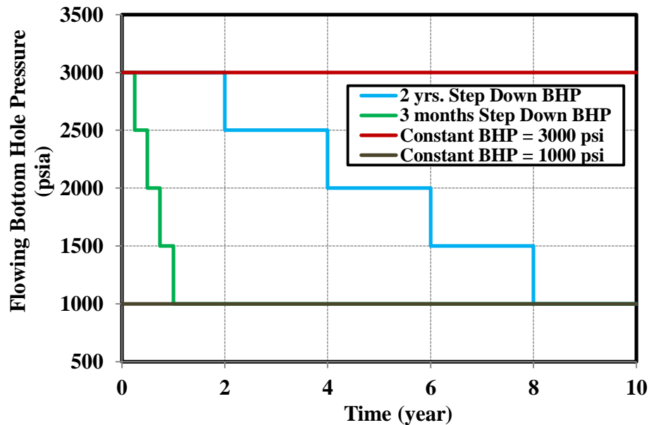
Fig. 13. Various well operating strategy to control production.
